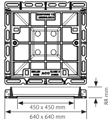
Rhinocast Square Infill Access Cover (Class D) part # 143029
