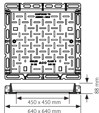
Rhinocast Square Infill Access Cover (Class D) part # 143029
