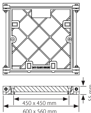
Rhinocast Square Infill Access Cover (Class B) part # 85014
