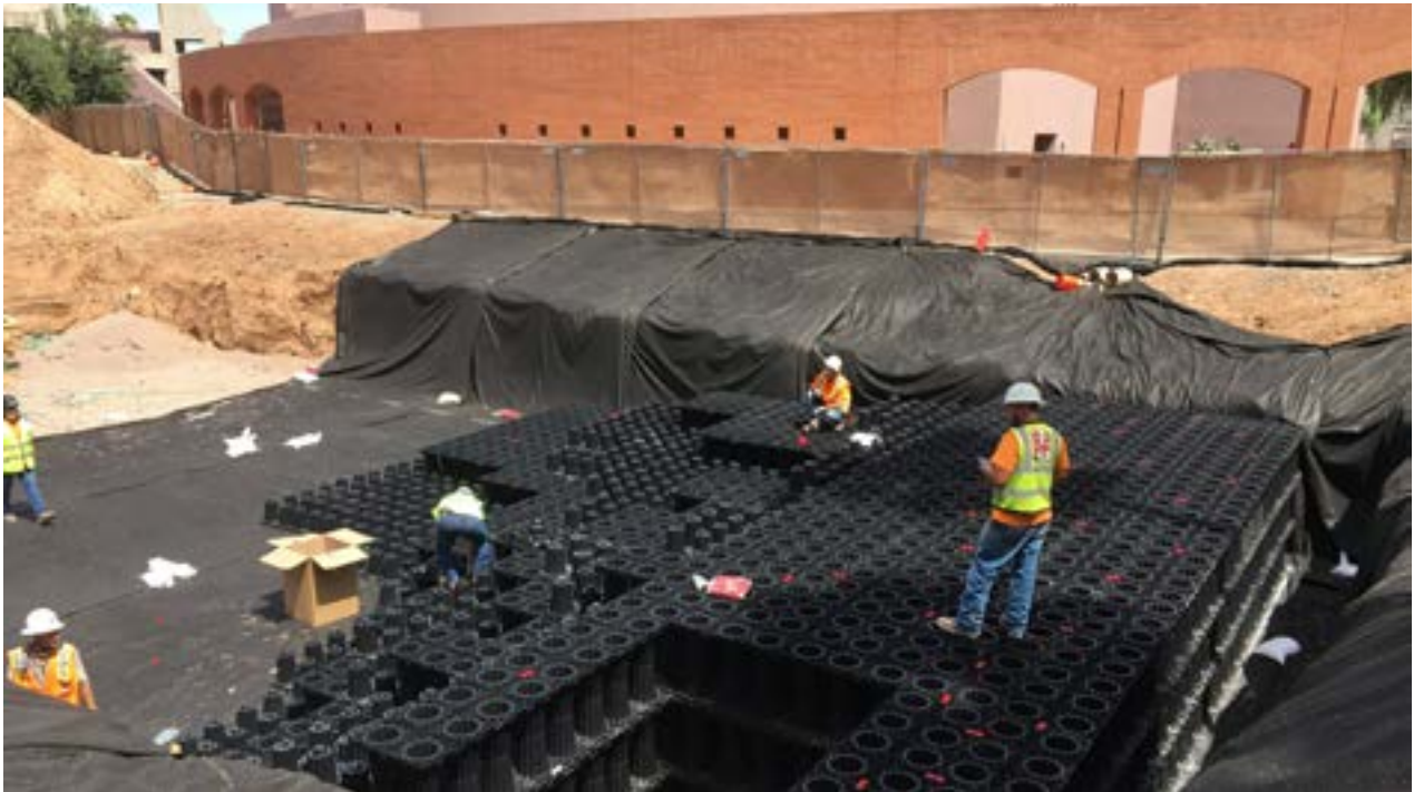
During Phase 2 of the project the ACO StormBrixx® 600 HD retention system was used at the University's Nelson Fine Arts Center.
