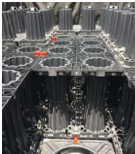
Units snap-lock together in a brick-bonding pattern.
